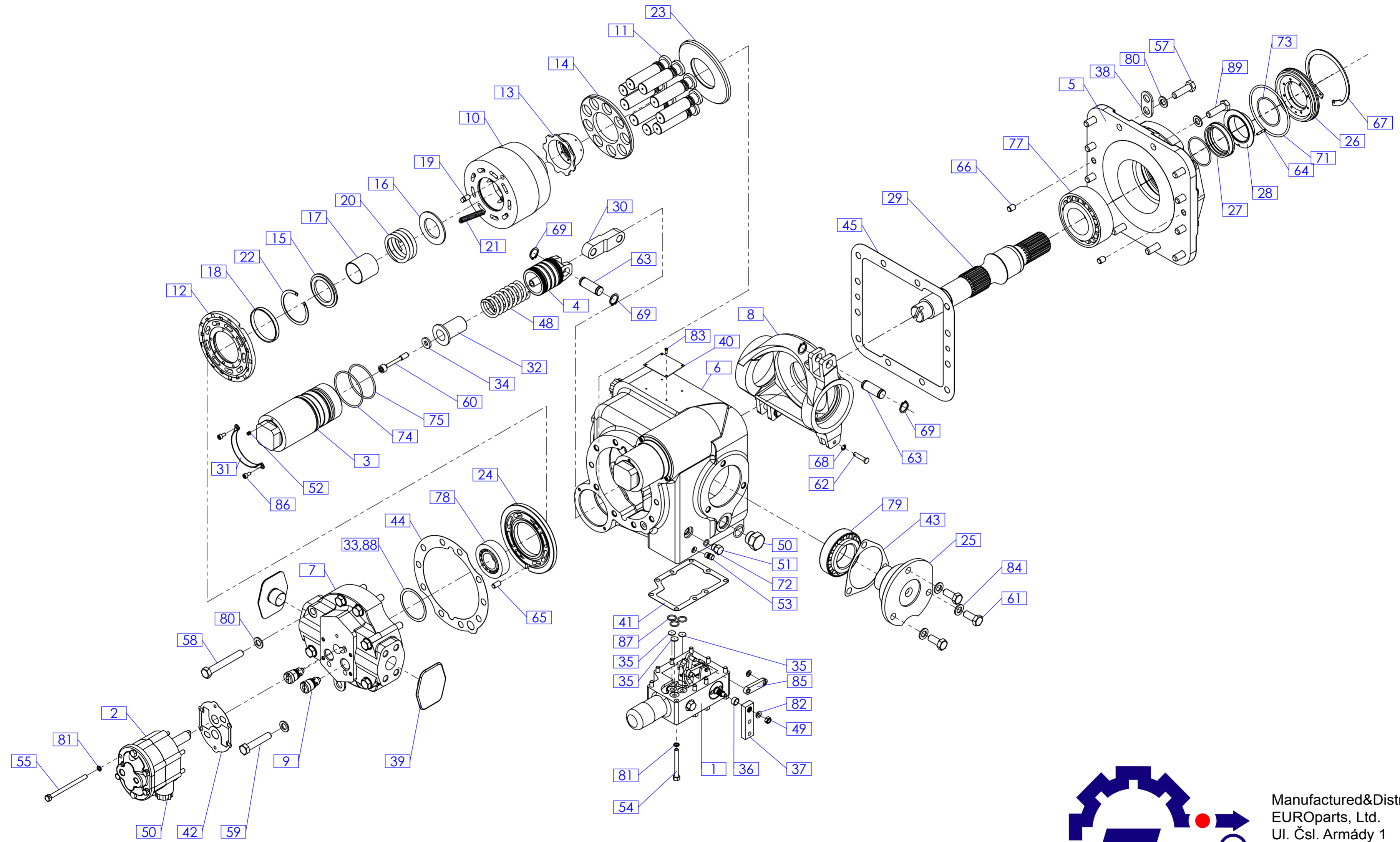
Axial Piston Variable Displacement Pump – Explosion View
